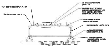
1 CABLE TRAY NOT TO SCALE
