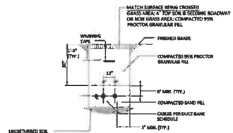
1 DIRECT BURIAL DUCT BANK NOT TO SCALE
