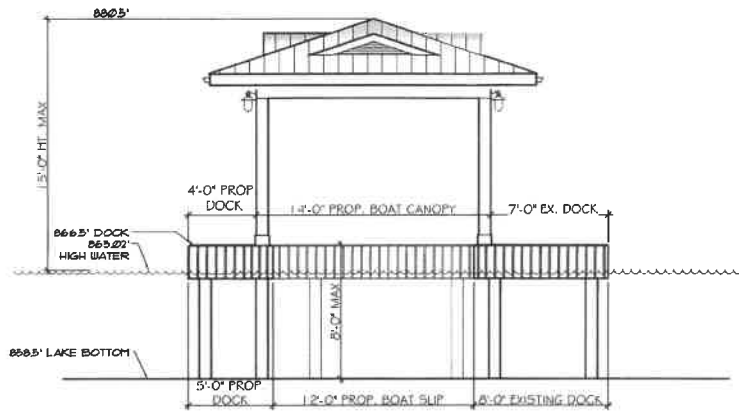
EAST ELEVATION 3/16" = 1'-0"
