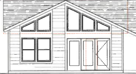
NORTH-EAST ELEVATION 3/16"=1'-0"
