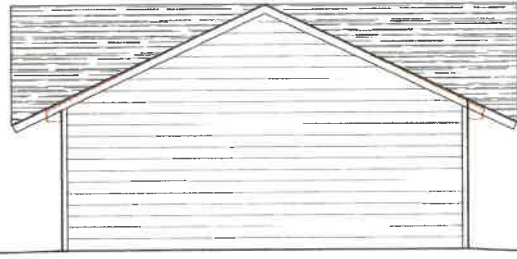
SOUTH-EAST ELEVATION 3/16"=1'-0"
