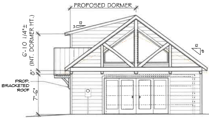
NORTH ELEVATION 3/16" = 1'-0"
