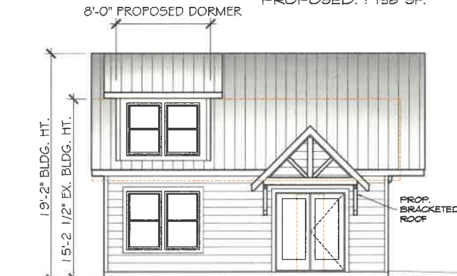
EAST ELEVATION 3/16" = 1'-0"
