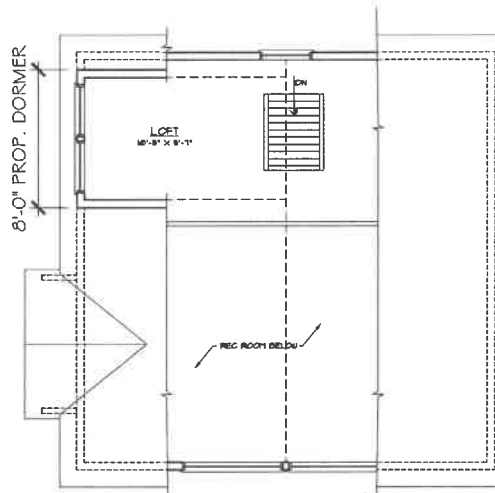
LOFT PLAN 3/16" = 1'-0" EXIST. : 198 SF. PROPOSED. : 198 SF.
