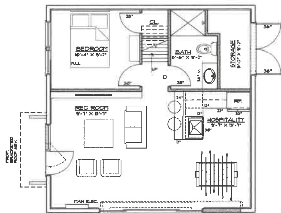
FIRST FLOOR PLAN 3/16" = 1'-0" 589 SF.
