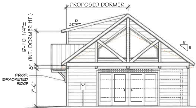
NORTH ELEVATION 3/16" = 1'-0"
