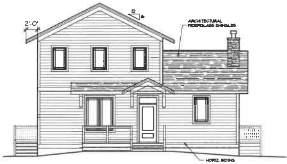
WEST ELEVATION 1/8" = 1'-0"
