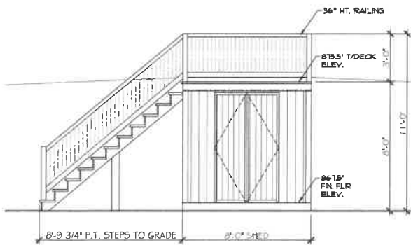
EAST ELEVATION 1/4" = 1'-0"
