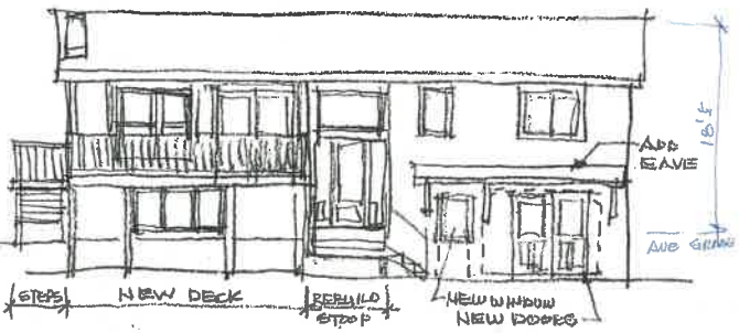
EAST ELEVATION 1/8" = 1'-0"
