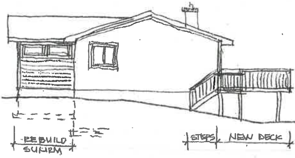
SOUTH ELEVATION 1/8" = 1'-0"
