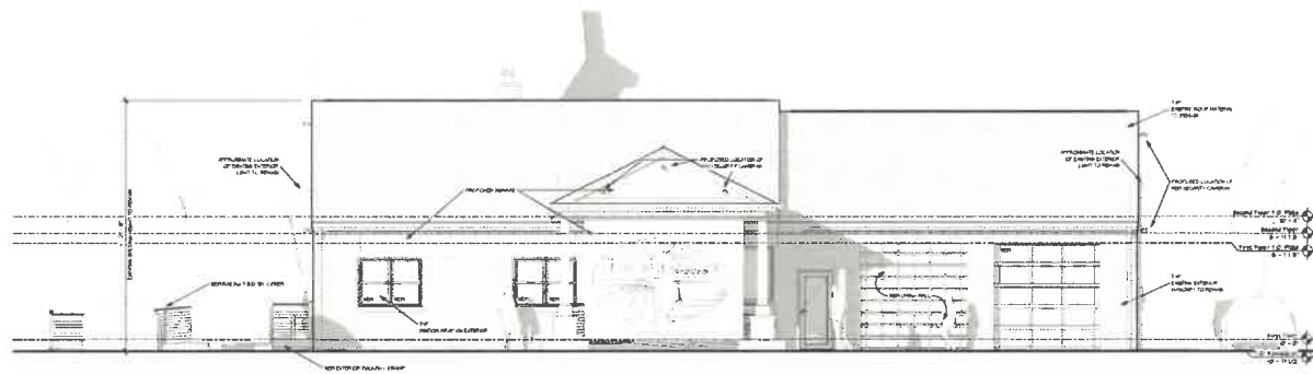
123 Building Elevation - South Scale: 1/8" = 1'-0"
